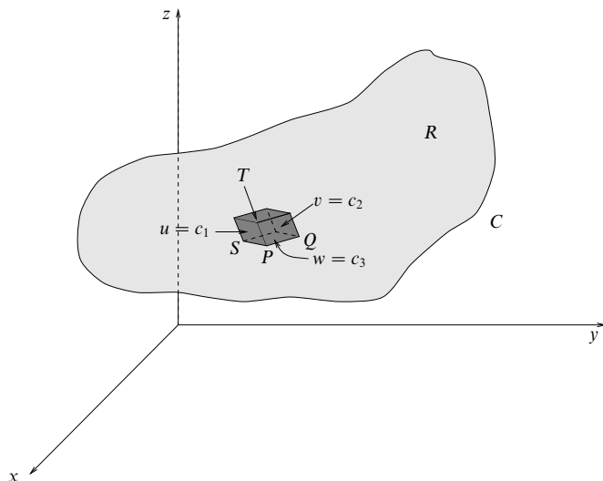
Figure 6.12 A three-dimensional region of integration R , showing an element of volume in u, v, w coordinates formed by the coordinate surfaces u = \text{constant} , v = \text{constant} , w = \text{constant} .
